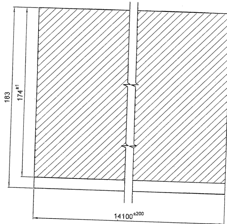
Graphite thickness -160 Micron
